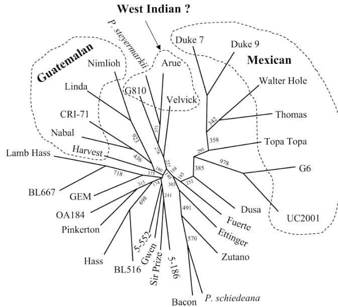
Figure 4-2. Results of molecular analysis by Ashworth and Clegg (2003): “Neighbor-joining consensus tree of 1,000 bootstrap replicates generated from allele frequencies at 25 microsatellite loci for 33 avocado genotypes. Many bootstrap values are low, reflecting the large number of hybrid cultivars in the data set. Dotted lines surround genotype assemblages belonging to the three botanical races of avocado—Guatemalan, Mexican, and West Indian. The West Indian cluster is assigned based on cv. Arue, whose ancestry is presumed to be West Indian. Intermediate clusters unite genotypes of various hybrid origins.”
