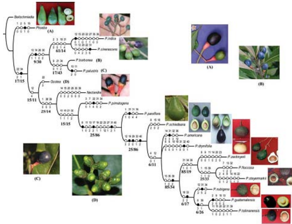
Figure 4-1. Phylogenetic analysis of Neotropical Persea from Rojas et al., 2007: “Strict consensus of the five equally parsimonious trees for Persea taxa based on morphological characters. Length = 181, consistency index = 39 and retention index = 60. Synapomorphies are black circles and homoplasies are open circles. Bootstrap/jackknife percentages are given below branches”
